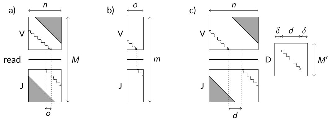
Figure 4 – V(D)J designation by dynamic programming, declared in segment .h . See Jones and Pevzner (2004, chapter 6) for an introduction on dynamic programming methods to compare sequences. Grayed out triangles show parts excluded from the computation. a) Search of the best alignments between the read with a V gene and a J gene, in O(Mn) time, where M is the total size of indexed genes and n the size of the read. Candidate V and J segments are independently predicted. b) When the best alignments make the candidate V and J segments overlap on o \leq n positions, the best split point is found by another search in time O(mo) , where m \ll M is the total size of considered V and J genes. c) In the case of a VDJ-like recombination, the central segment is predicted by a local alignment in time O(M'(d + 2\delta)) , where M' is the total size of indexed D genes and d + 2\delta \leq n is the size of the zone where the D segment is searched. Overlaps between V and D or between D and J candidate segments are handled as previously. The algorithm finally runs in time O((M + M')n) .
