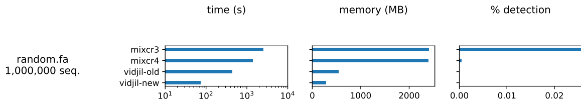
Figure 5. Detection results of MiXCR and Vidjil-algo on random sequences (dataset A)
