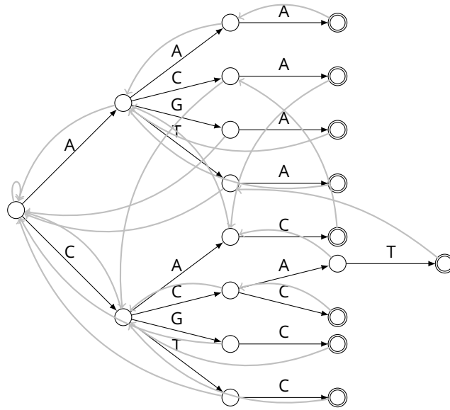
Figure 2. Aho-Corasick automaton for P(\text{ACAC}, \#-\#) \cup P(\text{CCAT}, \####) , that is for the projected seeds A-A, C-C, and CCAT. The gray arrows correspond to the failure transitions in the Aho-Corasick automaton. They can be seen as \varepsilon -transitions and are removed in a pre-processing step, without changing the number of states.
