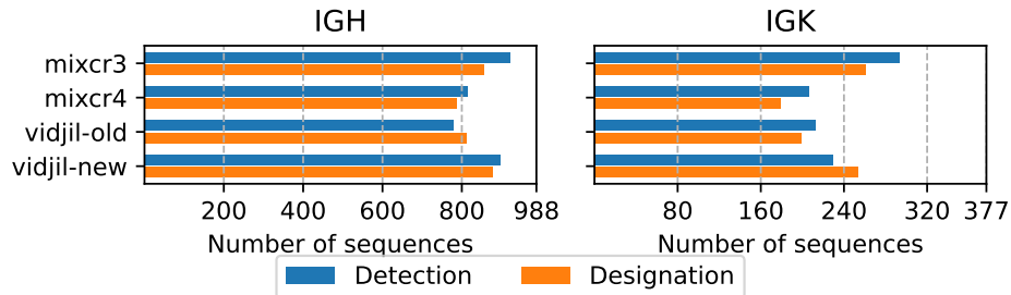
Figure 8. Correct detection and designation of V(D)J recombinations on LIGM-DB version LIGMDB_V12 (dataset D) with MiXCR and Vidjil-algo.
