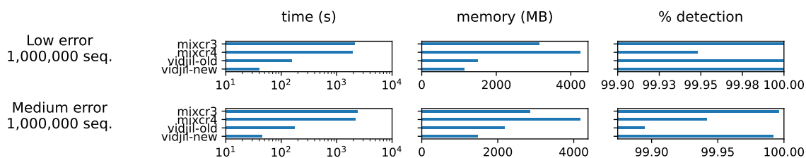
Figure 7. Detection on Afzal et al. (2019) TRB benchmark (dataset C) by MiXCR and Vidjil-algo.
