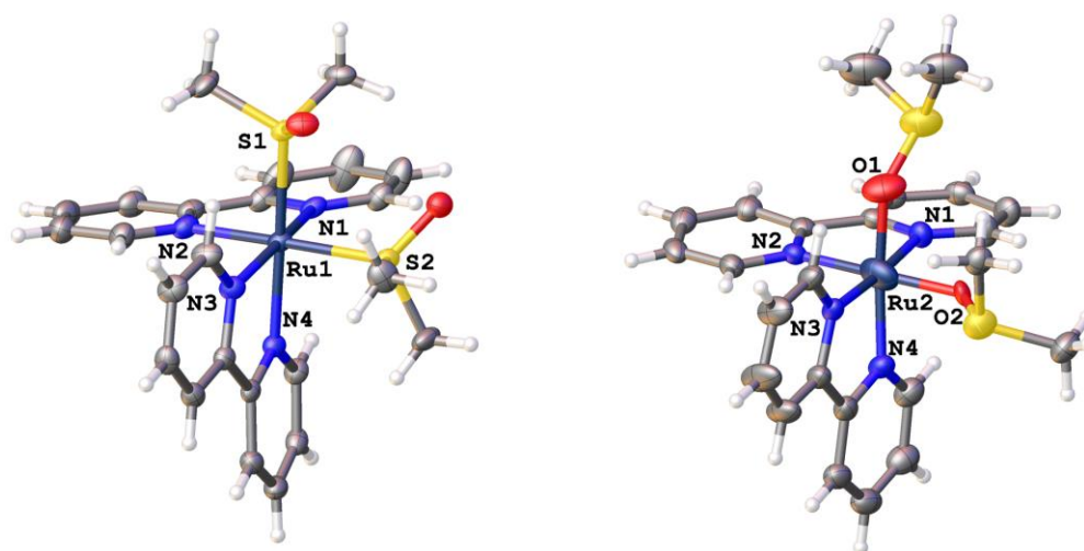
Figure 1. Ground state structure of [\text{Ru}(\text{bpy})_2(\text{dmsO})_2]^{2+} (left). Isolated molecular structure of bis-[O,O]- [\text{Ru}(\text{bpy})_2(\text{dmsO})_2]^{2+} after irradiation with 405 nm light (right). Ruthenium, navy; nitrogen, blue; oxygen, red; sulfur, yellow; carbon, grey; hydrogen, white.
