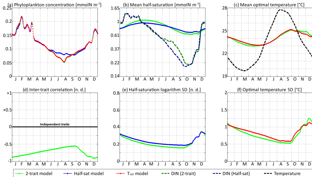
Figure 10. SPEAD state variables at the surface for \nu_x = 0.00001 and \nu_y = 0.0001 \text{ } ^\circ\text{C}^2 (low mutation rates) compared with the state variables of one-trait models: (a) total phytoplankton concentration, (b) (geometric) mean half-saturation, (c) mean optimal temperature, (d) inter-trait correlation, (e) half-saturation logarithm standard deviation, and (f) optimal temperature standard deviation. The dashed lines represent the environmental drivers.
