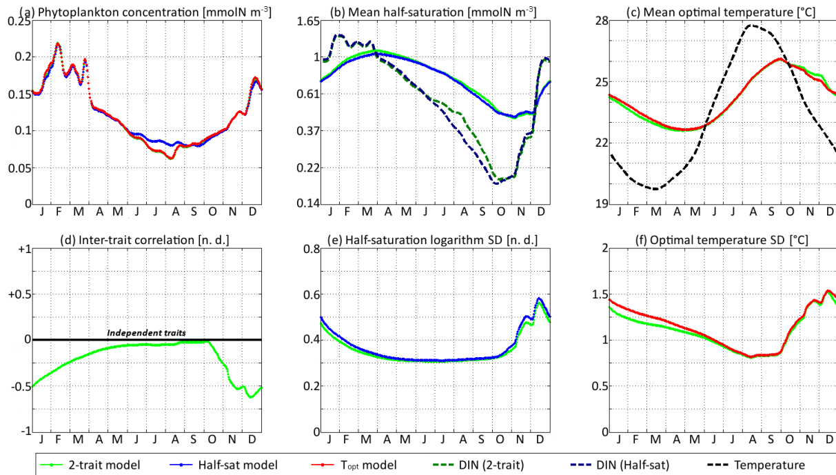
Figure 9. SPEAD state variables at the surface for \nu_x = 0.001 and \nu_y = 0.01 \text{ } ^\circ\text{C}^2 (standard) compared with the state variables of one-trait models: (a) total phytoplankton concentration, (b) (geometric) mean half-saturation, (c) mean optimal temperature, (d) inter-trait correlation, (e) half-saturation logarithm standard deviation, and (f) optimal temperature standard deviation. The dashed lines represent the environmental drivers.
