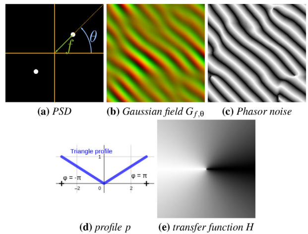
Figure 3: Phasor noise. The power spectrum distribution (PSD) (a) fully controls a complex Gaussian field (b). The profile function (d) (triangle profile here) defines the transversal shape of the waves. The resulting field of profiled wave field (c) can be equivalently expressed as (i) the composition of the profile p with the argument of the Gaussian field G_{f,\theta} , or (ii) the composition of a 2D transfer function H (shown in (e), equal to p \circ \text{atan2} ) with the Gaussian field G_{f,\theta} itself [GSDT22].
