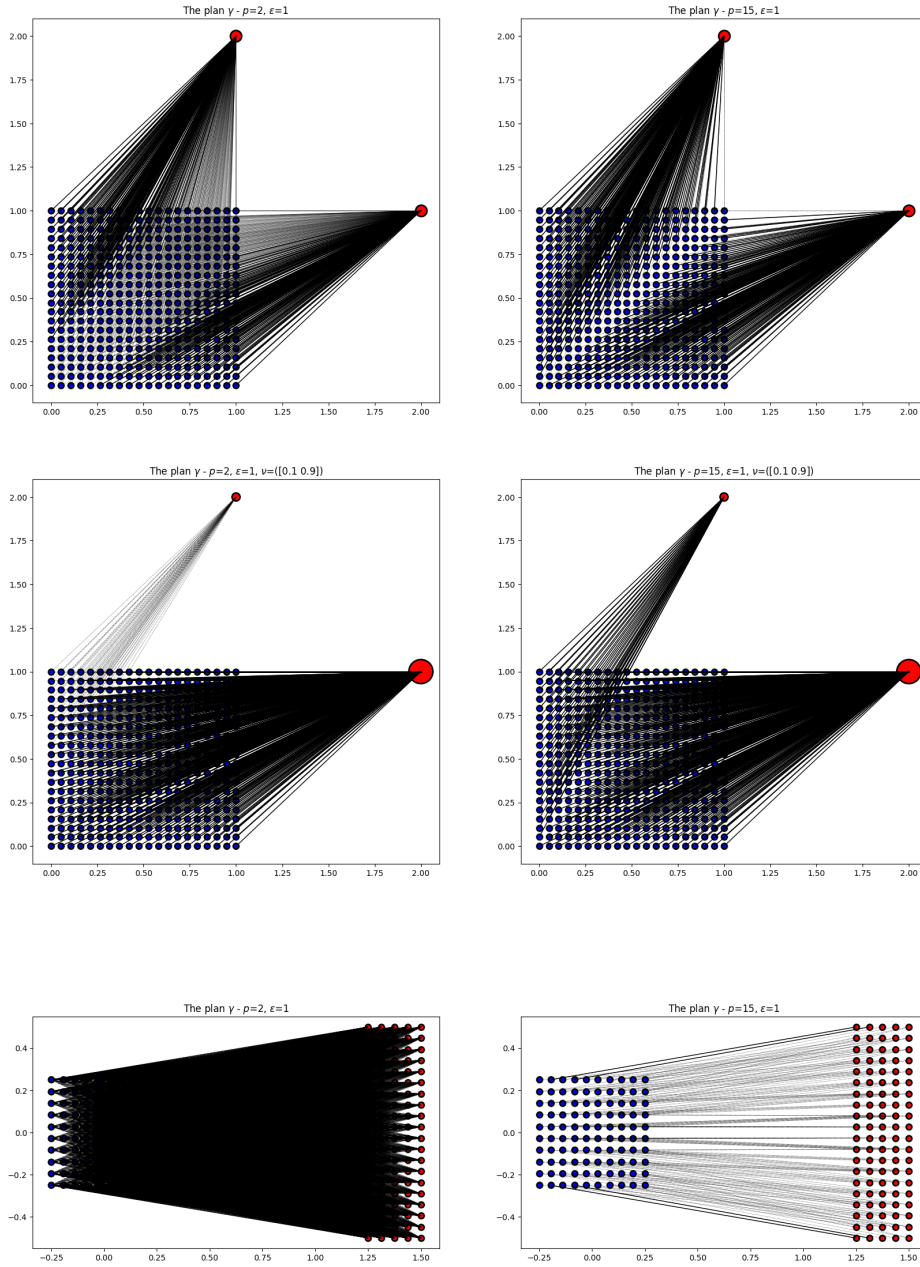
Figure 4: Comparison among three different examples: \varepsilon = 1 , c(x, y) = |x - y|^p , on the left p = 2 , on the right p = 15 . On top: \mu a uniform discretization of the unitary square and \nu uniformly concentrated on the points (1, 2) and (2, 1) . In the middle: \mu the same discretization of the unitary square, \nu = 0.1\delta_{(1,2)} + 0.9\delta_{(2,1)} (the point (2, 1) is represented by a bigger dot). On bottom: \mu a uniform discretization of the square [-0.25, 0.25] \times [-0.25, 0.25] and \nu of the rectangle [1.25, 1.5] \times [-0.5, 0.5] .
