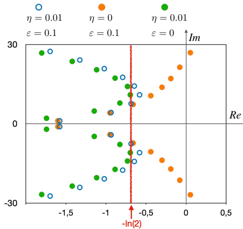
Figure 2: Spectrum of the closed-loop system: influence of viscosity on stability in case of parameter uncertainty.
