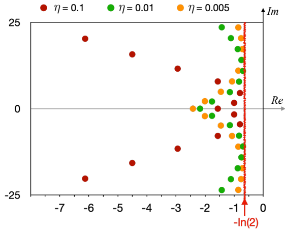
Figure 1: The spectrum of the closed-loop system for \eta = 0.005, 0.01 and 0.1 .
