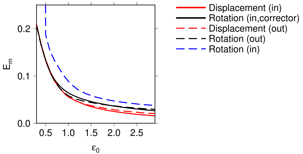
Figure 14. Error \bar{E}_m as a function of \epsilon_0 for V_S^* , which is derived from the FWI results, with correctors, using displacement (solid red) and rotational (solid black) receivers positioned within the heterogeneous area. Results from the other cases (dashed curves) are also shown for comparison.
