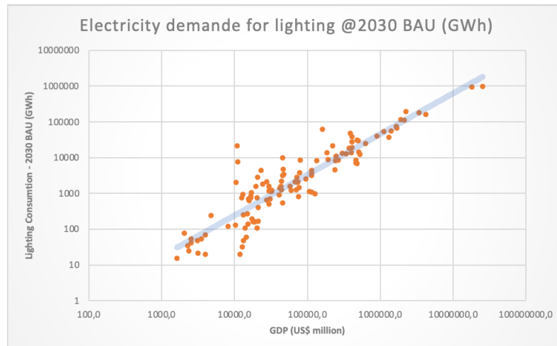
Figure 6: 2030 Electricity demand under BAU Scenario vs country's GDP. Energy data from [U4E-22]
