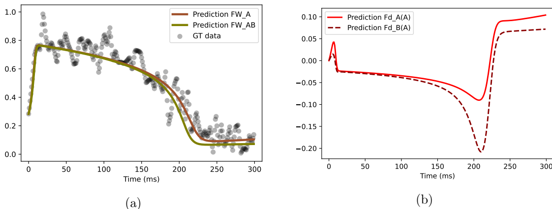
Figure 13: (a) Validation results of the framework for ROI A, with the following legend: Ground truth (GT) data, prediction of the framework (Prediction FW_A) trained on only ROI A data, and prediction of the framework composed of ( F_p ) component trained on ROI A data and DL ( F_d ) component trained on ROI B data (Prediction FW_AB). (b) Comparison of the DL component trained on ROI A data ( F_{d_A}(A) ) and on ROI B data ( F_{d_B}(A) ), applied on validation ROI A data.
