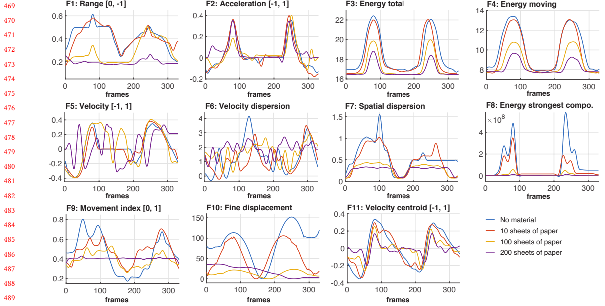
Fig. 5. Time series of the radar signal as the ball swings past the sensor. Each plot represents one Soli core feature for the baseline (no material) condition and 3 different thicknesses of Paper material (10, 100, and 200 sheets of paper). See our Supplementary Materials for additional results.
