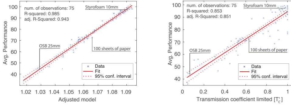
Fig. 8. Linear regression models to predict gesture classification performance. Left: multi-predictor model using 54 high-correlation Soli core features and material meta-features, marked in bold in Figure 7. Right: single-predictor model using T'_c of core feature Energy Total (F3).
