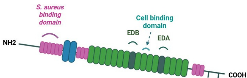
Figure 3. Schematic representation of fibronectin monomer. Binding sites for Staphylococcus aureus bacteria and the integrin \alpha 5 \beta 1 /cell-binding domain are reported. The extra domain A (EDA), which is involved in matrix remodeling, and the extra domain B (EDB), which has an important role during embryogenesis, are also indicated.
