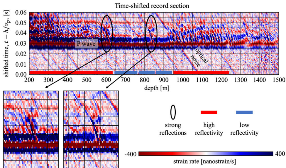
Figure 6. Time-shifted section of shot 1 fired close to the borehole at \Delta = 43 m. Each trace is shifted by h/v_p , where h is depth and v_p = 3800 \text{m s}^{-1} is an approximate average P wave speed. The section is centred around the direct P -wave arrival. Depth intervals where strong reflected waves are visible are marked by horizontal bars. Blue bars mark depth intervals where strong reflections are essentially absent. Black ellipses with zoomed panels indicate easily visible individual reflections. Optical noise has an apparent propagation speed of exactly v_p = 3800 \text{m s}^{-1} and corresponds to the purely vertical striping in Fig. 3.
