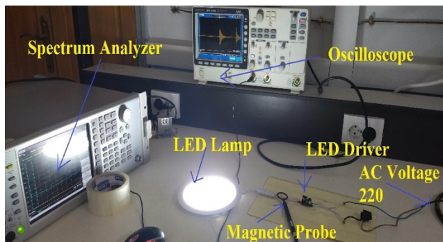
Fig. 3. Bench measuring the near magnetic field with and without shielding above the driver.
