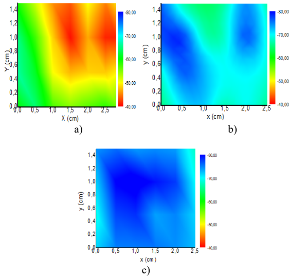
Fig. 9. Magnetic field scan component H_z above the LED driver at z = 1.5 cm: (a) without shielding, (b) partial shielding (c) total shielding.
