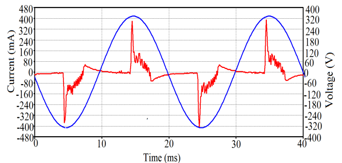
Fig. 5. Input current and voltage for LED Driver.
