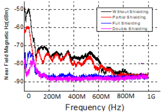
Fig. 13. Near magnetic field with and without Shielding at the center of LED Driver at z = 1.5 cm, measured with the probe RSH400-1.
