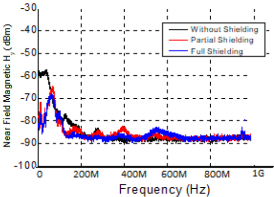
Fig. 11. Near magnetic field of component H_y with and without shielding
