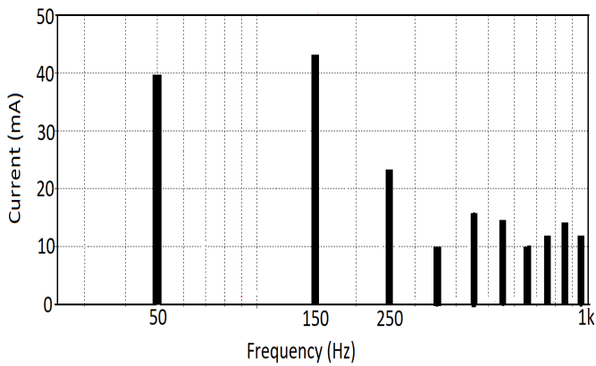
Fig. 6. Frequency spectrum of harmonics generated by the AC/DC LED Driver.
