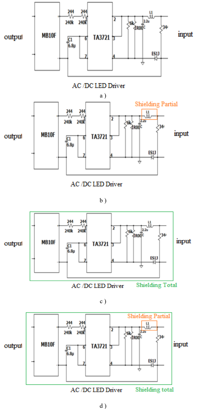
Fig. 8. LED driver and type of Shielding a) without Shielding, b) Partial shielding, c) Total shielding, d) Double shielding.
