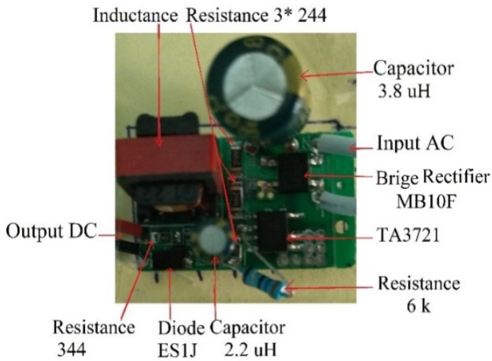
Fig. 1. LED driver modules integrated onto the PCB.
