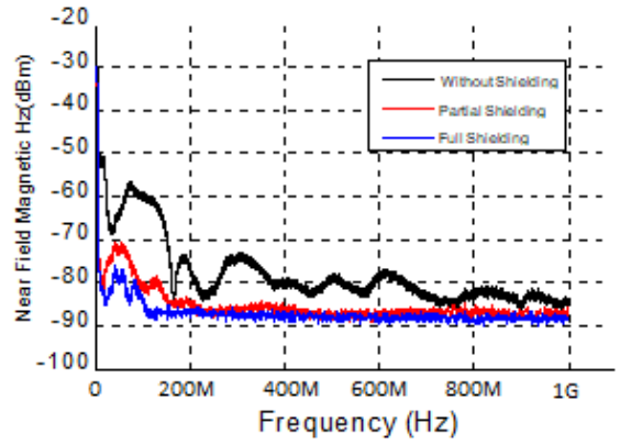
Fig. 12. Near magnetic field of component H_z with and without shielding.
