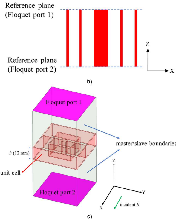
Figure 1. The proposed unit cell. a) 3D view. b) Sectional view. c) Simulation setup.
