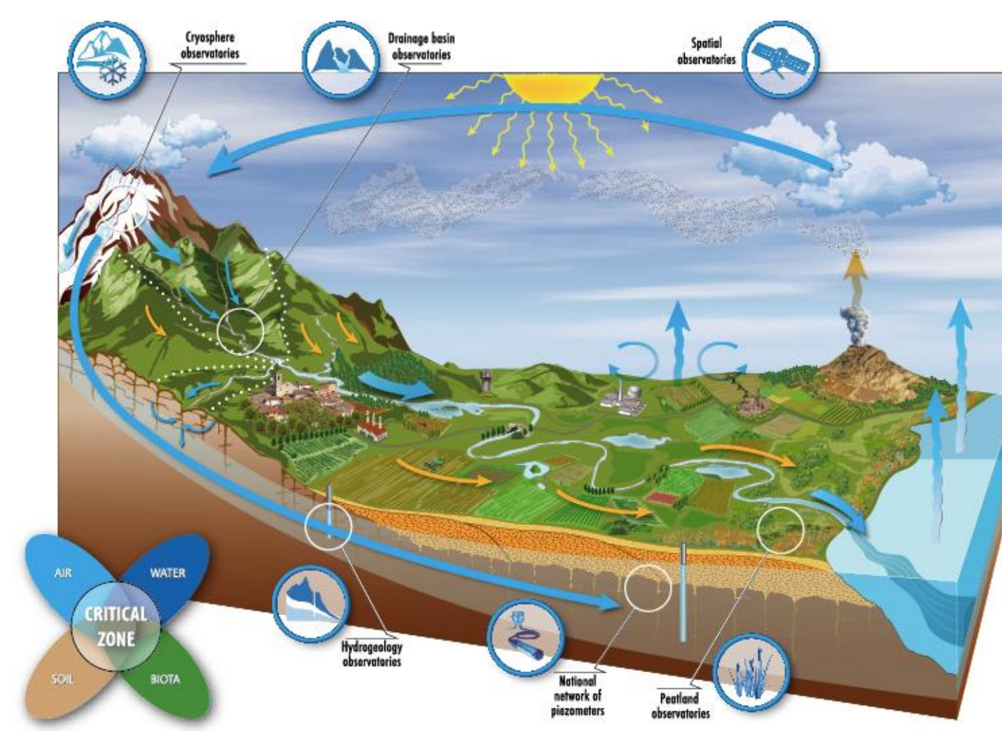
Figure 2: Schematic view of the critical zone with the various sampled compartments and objects @ Jo el Dion, IPGP
