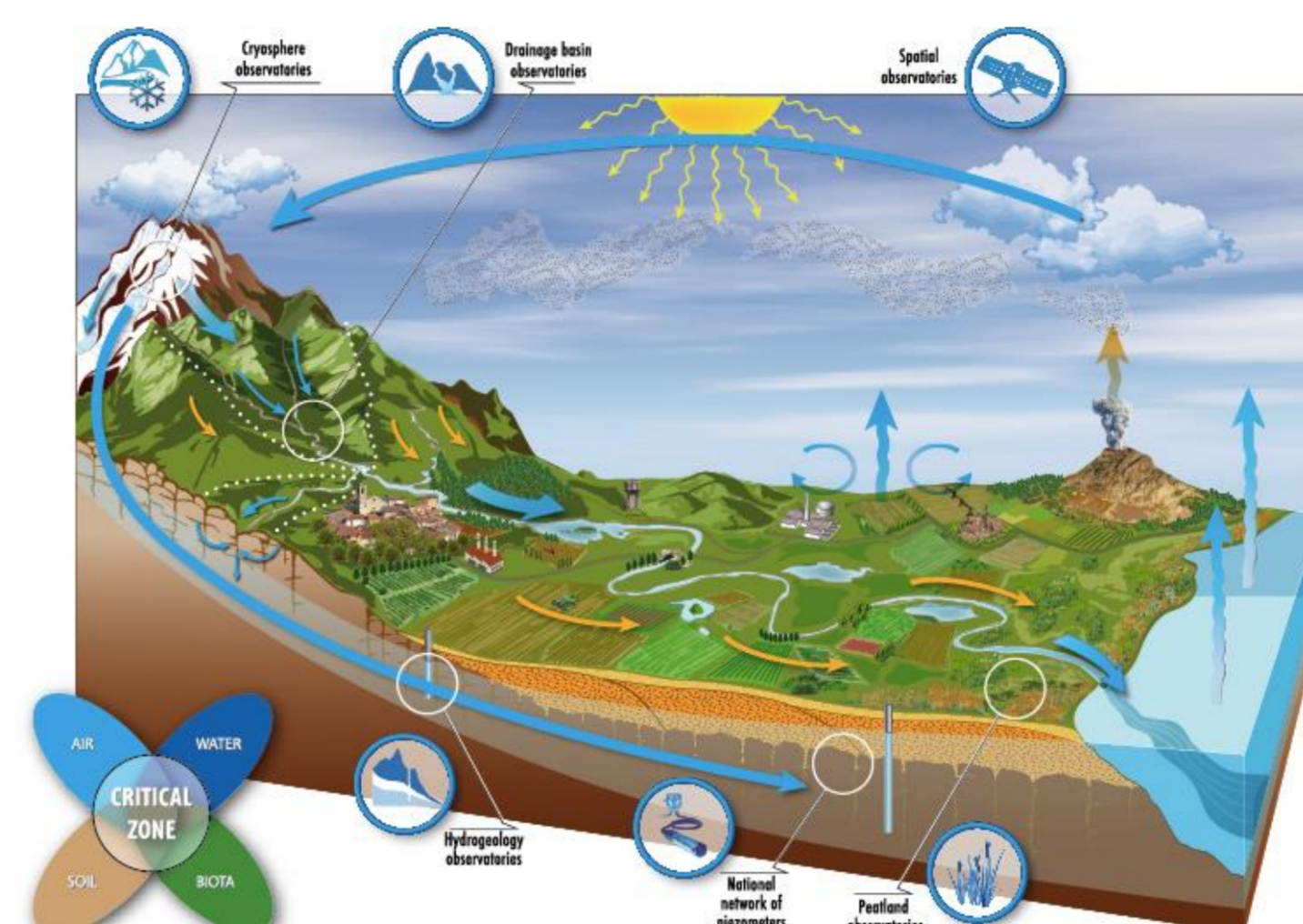
Figure 2: Schematic view of the critical zone with the various sampled compartments and objects @ Jo l Dion, IPGP
