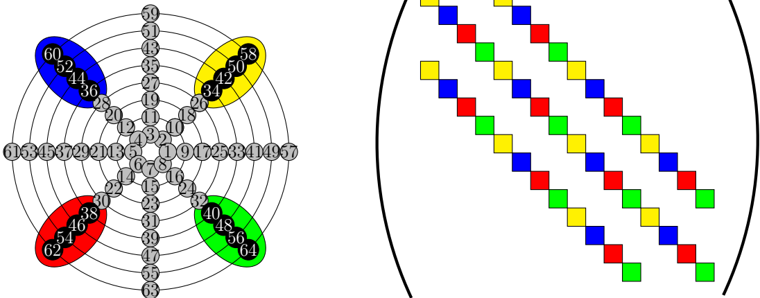
Fig. 4: Left: Circular mesh with 64 nodes as in Figure 3 (right). Without loss of generality, we assume a circle-wise global numbering. Focus on black colored nodes of the radial smoother. Different grid lines of the smoother given by different background colors. Right: Nonzero pattern of the submatrix A_{R_B R_B} when using a compact five, seven, or nine point stencil, with colors referring to the particular grid lines as depicted on the left figure. Different numberings of the nodes lead to different nonzero patterns.
