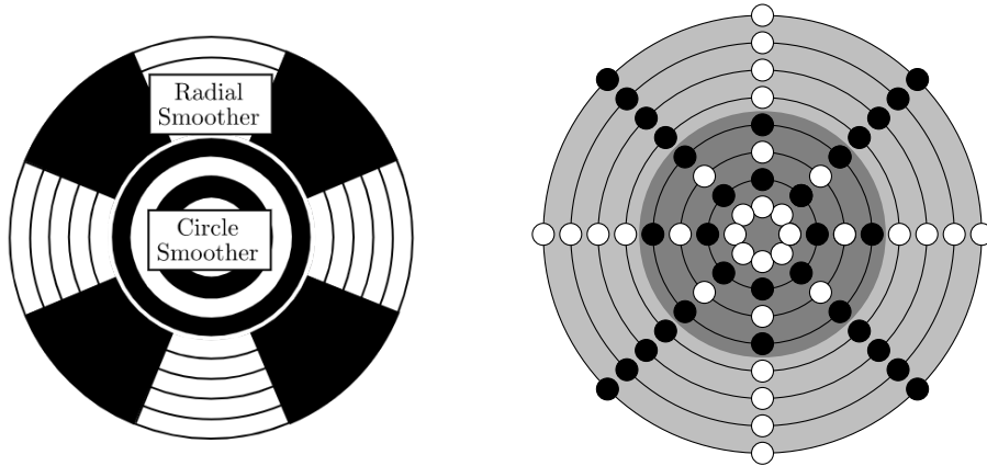
Fig. 3: Left: Schematic subdivision of a circular domain into an interior subdomain where circle-line smoothing is used and an exterior subdomain where radial smoothing is used. Right: Circular mesh with 64 nodes. Circular smoothing applied on the four interior circles (dark gray background color), radial smoothing applied on the four exterior circles (light gray background color). Nodes colored according to smoother color.
