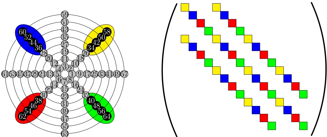
Fig. 4: Left: Circular mesh with 64 nodes as in Figure 3 (right). Without loss of generality, we assume a circle-wise global numbering. Focus on black colored nodes of the radial smoother. Different grid lines of the smoother given by different background colors. Right: Nonzero pattern of the submatrix A_{R_B R_B} when using a compact five, seven, or nine point stencil, with colors referring to the particular grid lines as depicted on the left figure. Different numberings of the nodes lead to different nonzero patterns.
