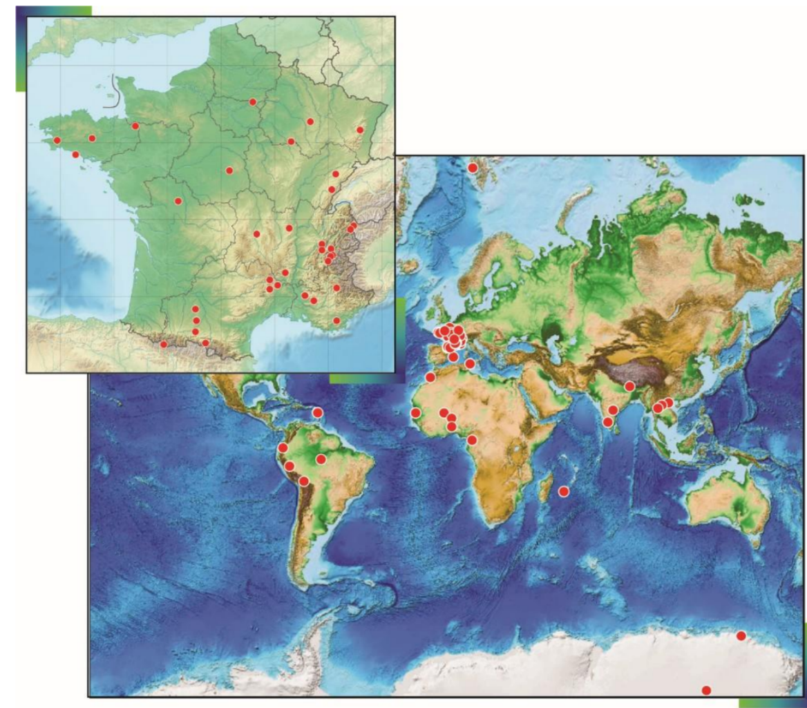
Figure 2: Location of the OZCAR RI observation sites (Gaillardet et al., 2018)
