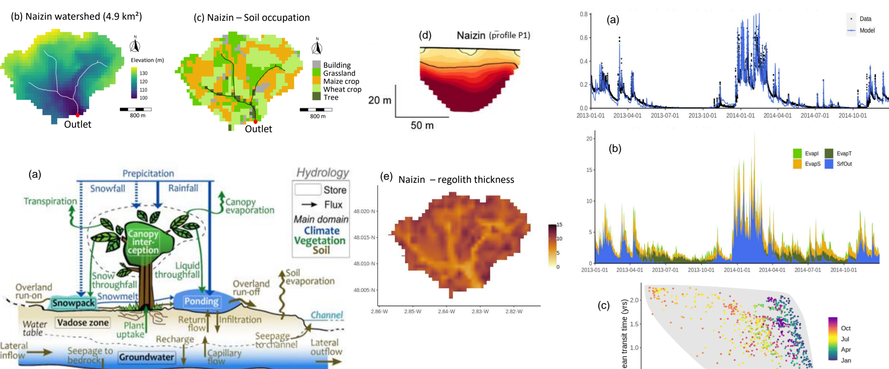
Figure 6: (a) Scheme of the E_cH_2O -Iso model (Kuppel et al., 2018 and of the input data for the Naizin watershed (AgrHys observatory); (b) topography, (c) land use, (d) a resistivity profile that was used to define the regolith depth (e) (figures from Ackerer et al., in preparation)
