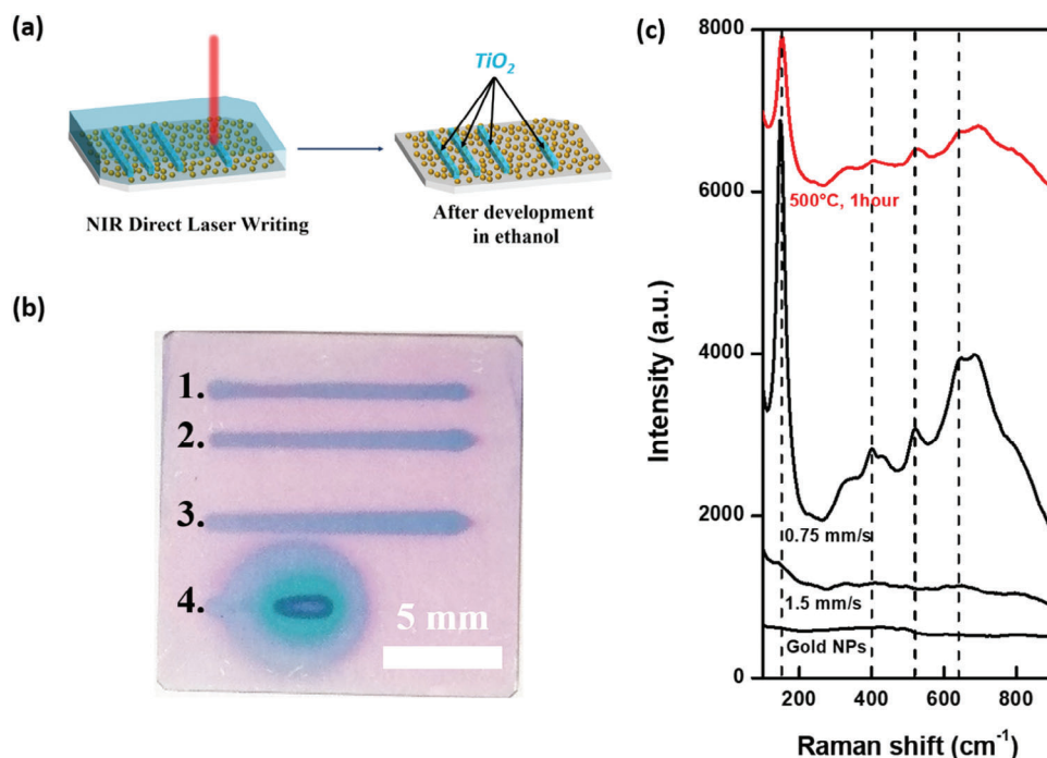
Figure 5. a) Schematic of direct laser writing process of crystalline \text{TiO}_2 on gold NPs by NIR and b) a picture showing lines obtained with a writing speed of 2 \text{ mm s}^{-1} at 11 \text{ kW cm}^{-2} (b1) and of 2 \text{ mm s}^{-1} (b2), 1.5 \text{ mm s}^{-1} (b3) and 0.75 \text{ mm s}^{-1} (b4) at 13 \text{ kW cm}^{-2} . c) Raman spectra of gold NPs, lines (b3) and (b4), and \text{TiO}_2 obtained by fast thermal annealing at 500 \text{ }^\circ\text{C} are plotted.
