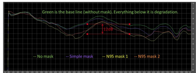
Fig 2. Output SPL level differences (in dB) for different types of medical mask shown in Fig 1 [5].
