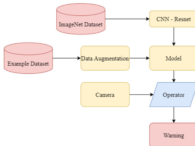
Fig. 2: Model flowchart
