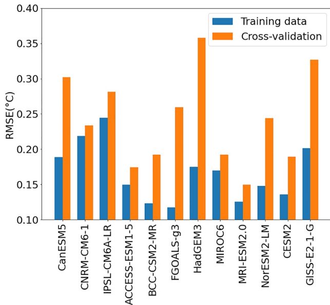
Figure 4. Root mean square error between the convolutional neural network output and the global mean surface air temperature of HIST, in °C, when using (blue bar) the training data and (cross validation, orange bar) when using the data of a model left out in the training.
