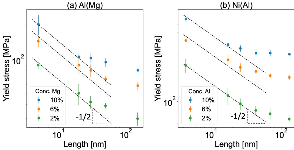
Figure 8. Average yield stress of edge dislocations in (a) Al(Mg) and (b) Ni(Al) solid solutions measured by atomistic simulations. Mean yield stresses and standard deviations were obtained by sampling from five different cells.
