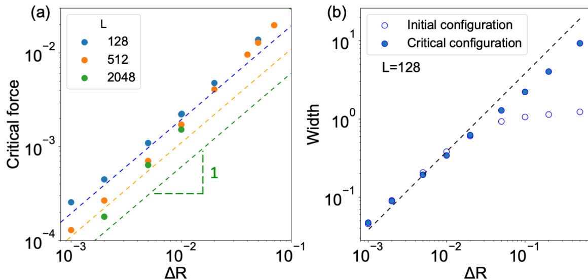
Figure 3. Average critical force (a) and dislocation width (b) as a function of noise amplitude \Delta R . Panel (a) is a zoom of Fig. 2 in Region I. The dashed lines are predictions from Larkin model (Eq. (5)). In (b), the dislocation width \omega is shown for L = 128 in the initial and critical configurations. The dashed line is the prediction from Larkin model (Eq. (8)).
