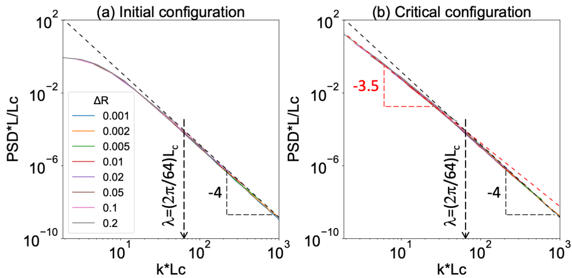
Figure 5. Scaled power spectral density (PSD) of dislocation heights in the (a) initial and (b) critical configurations. The same data are shown as in Fig. 4 but with the k -vectors scaled by 1/L_c and the PSDs scaled by L_c/L . The dashed black line in (a) and (b) is the prediction from Larkin model, which is expressed in scaled form as \overline{\text{PSD}} = 1440/\tilde{k}^4 . The red dashed line in (a) is a numerical fit.
