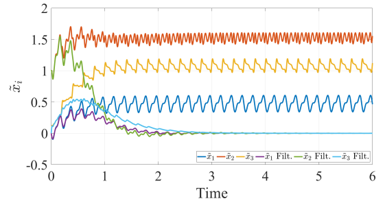
Figure 3: Evolution of the state-estimation error without (blue, red, yellow) and with (purple, green, cyan) internal model filter.
