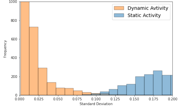
Fig. 5: Distribution of standard deviation ( std ) of magnitude |A| of the accelerometer signal
