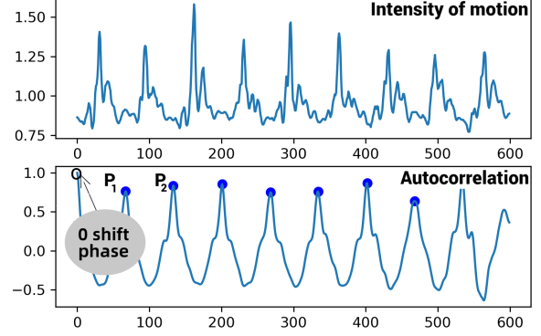
Fig. 2: Accelerometer magnitude |\mathbf{A}| and the corresponding ACF signal
