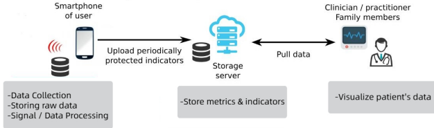
Fig. 1: Global application architecture
