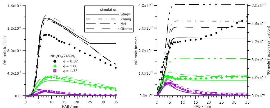
Fig. 1. Experimental and simulated NO and OH mole fraction profiles in NH_3/O_2/N_2 flames at p=10 kPa
