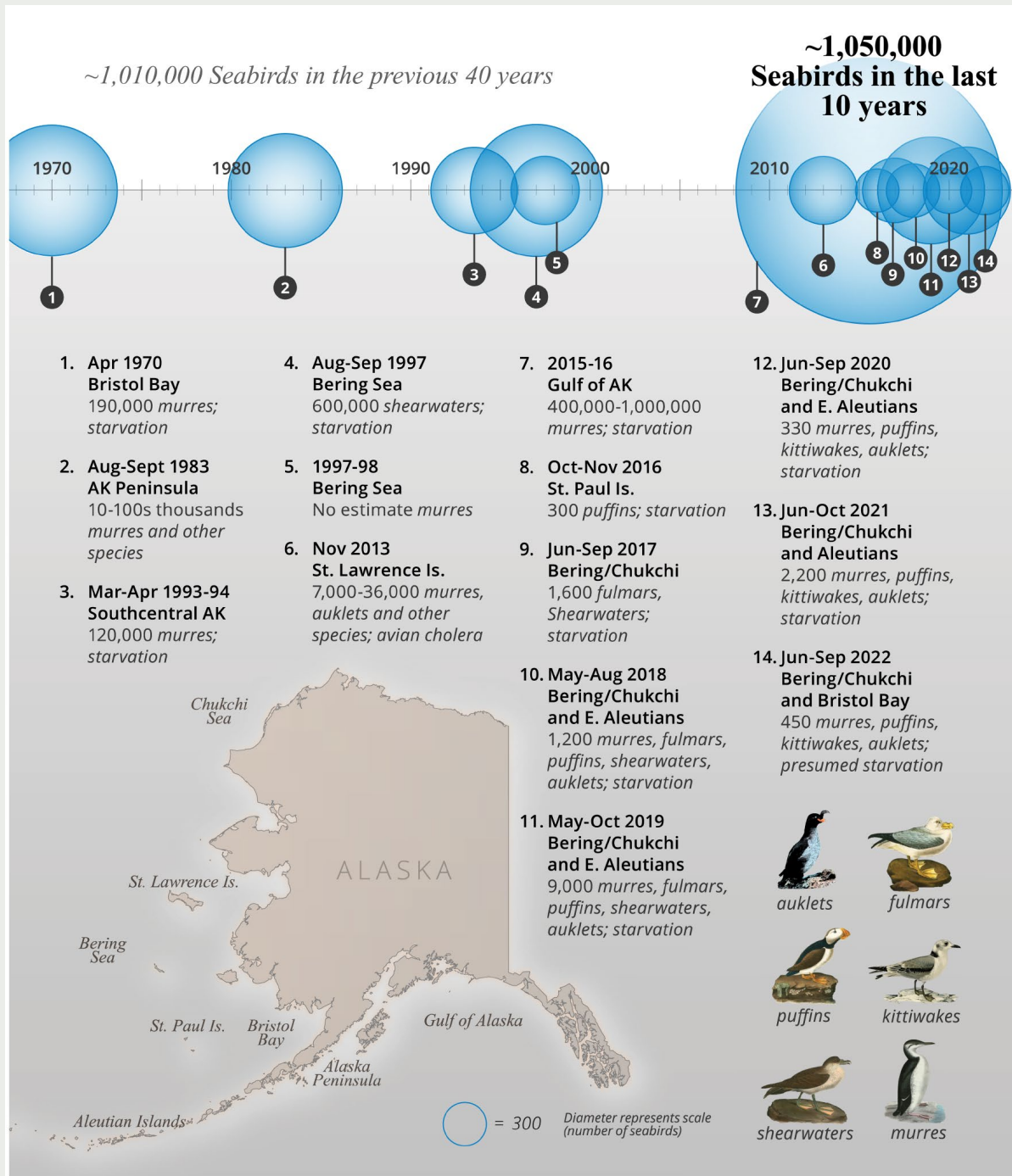
Fig. SB5.4 Alaska seabird die-offs, 1970 to present. Since 2015, mass die-offs have annually occurred in the northern Bering and southern Chukchi sea region. Species primarily affected include murre, puffin, auklet, shearwater, fulmar, and kittiwake.
