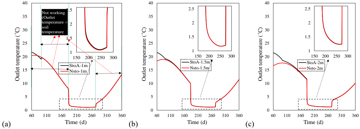
Fig. 6 Outlet temperature comparison of the storage scenario (ambient temperature) and the non-storage scenario for three installation depths a) 1m, b) 1.5m and c) 2m.
