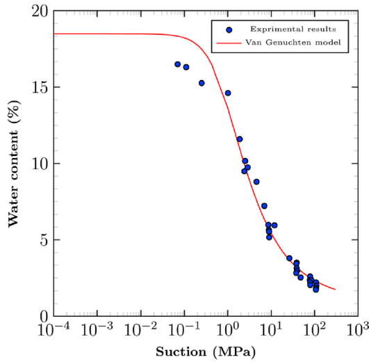
Fig. 1. SWRC of the studied backfill soil at the reference compaction state (dry density = 1.72 \text{ Mg.m}^{-3} )
