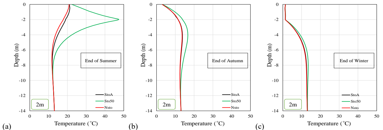
Fig. 8 Temperature profiles at the end of Summer (a), Autumn (b) and Winter (c)
