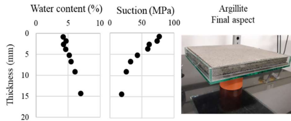
Fig. 6. Water content and suction measurements in the thickness of the Argillite sample at the end of the test I.
