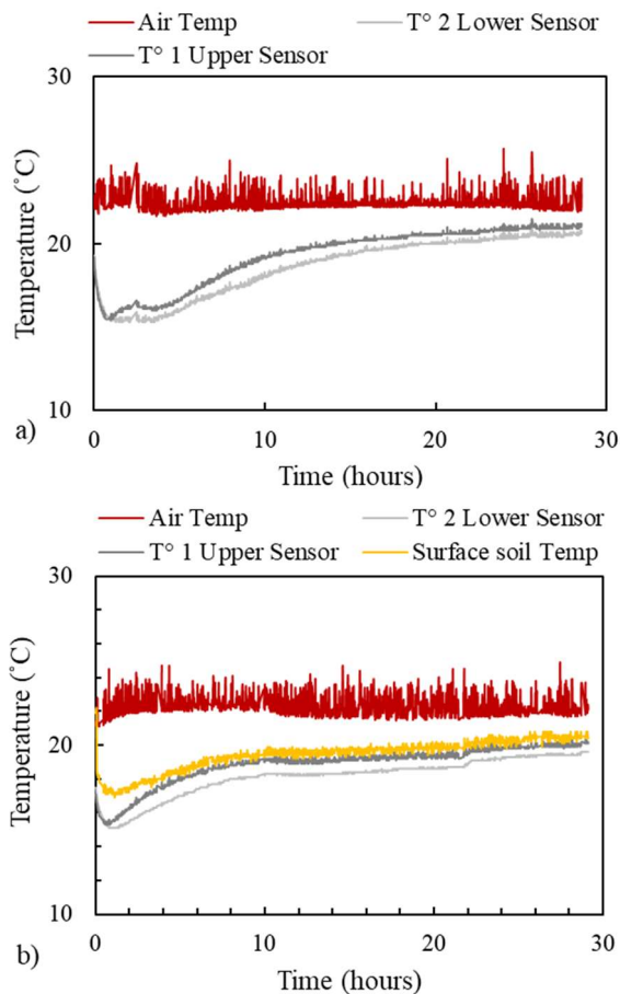
Fig. 9. Temperature evolution in different places of the samples a) A Test I, b) A-B mix, Test II.
