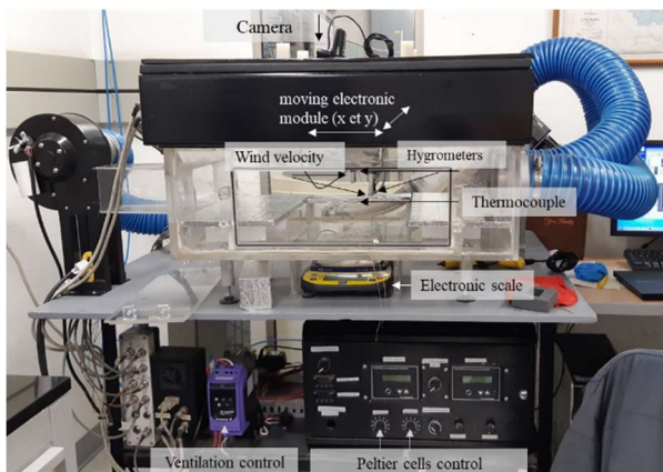
Fig. 1. General view of the climatic chamber.
