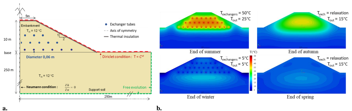
Figure 1: a. Embankment geometry and boundary conditions, b. Temperatures at the end of each season.
