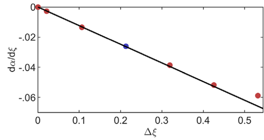
Figure 10. Evolution of the decay rate of the asymmetry parameter according to the fiber length \Delta\xi . The predictions of Equation (16) (solid black line) are compared with the results of the numerical integration of the NLSE (red circles). The blue circle corresponds to the parameter under study in this paper. The results are obtained for initial conditions \eta_0 = 0.75 , \alpha_0 = 0.15 and \phi_0 of 0.
