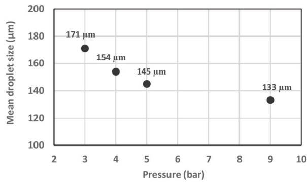
Fig. 5. Mean droplet diameter, i.e., D50 in µm (left) and mean droplet velocity, i.e., V50 in m/s (right) measured at 0.2 m distance below the injection point of one water mist nozzle.
