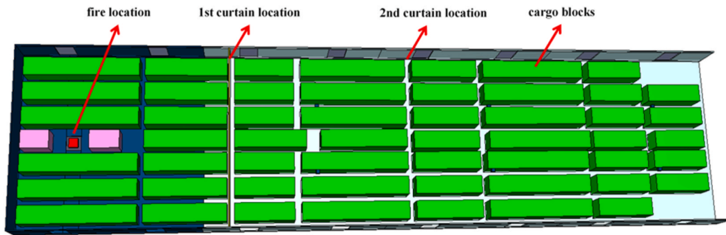
Fig. 28. Arrangement of cargo items in the fully loaded model deck.
