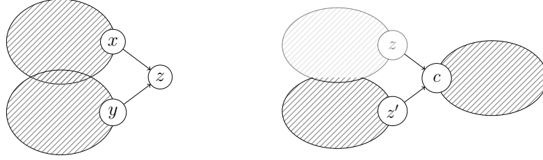
(a) First queried vertex \mathbf{z} is in B^\geq , and \mathbf{z} is bugged. (b) First queried vertex \mathbf{z} is in B^< , and \mathbf{z} is clean.
