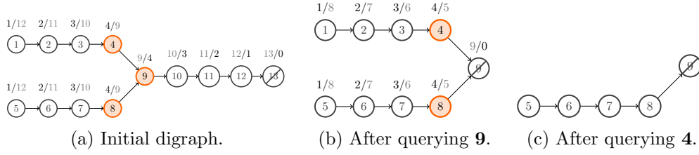
Figure 16: First two steps of golden bisection for a DAG of size 13.
