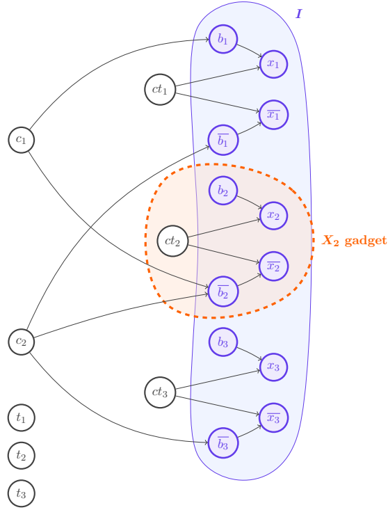
Figure 21: The graph resulting from the reduction of the formula (x_1 \vee \bar{x}_2) \wedge (\bar{x}_1 \vee \bar{x}_2 \vee \bar{x}_3) .
