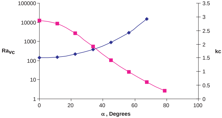
Fig. 3 Influence of the direction of the vibration on the values of the vibrational critical Rayleigh number Ra_v (left) and the critical wave number kc (right)
