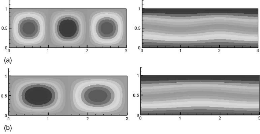
Fig. 4 Streamlines and isotherms for: (a) A_L = 3 , Ra_{Tnum} = 41 and Ra_{vnum} = 0 , (b) A_L = 3 , Ra_{Tnum} = 73 and Ra_{vnum} = 84
