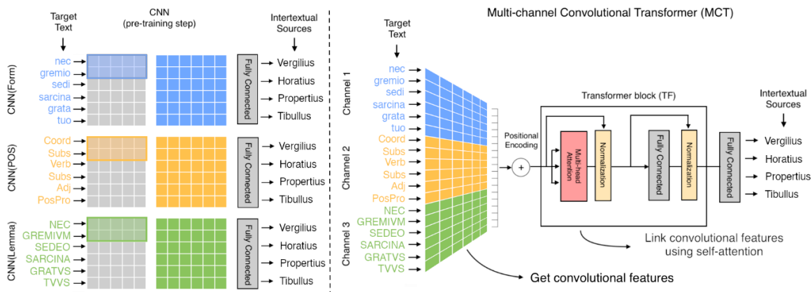
Figure 1. Multi-channel Convolutional Transformer
