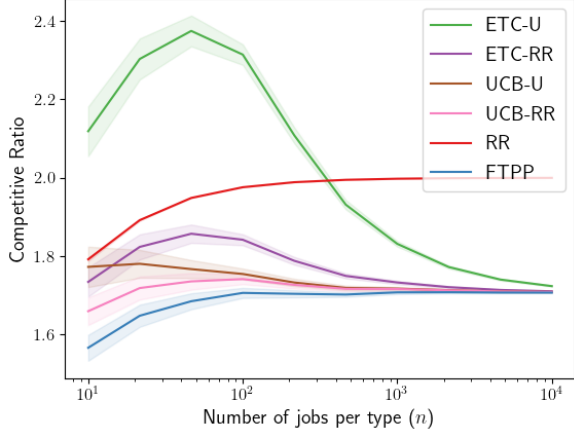
Figure 1. CR of all algorithms with varying number of jobs, \lambda_1 = 1 , \lambda_2 = 0.25 , averaged over 400 seeds.
