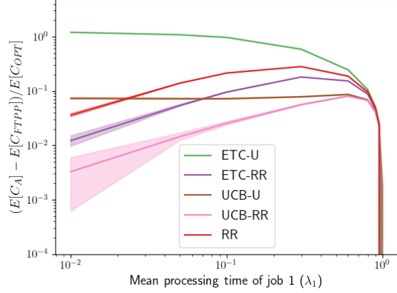
Figure 2. Normalized excess cost of all algorithms w.r.t. FTTP with varying value of \lambda_1 , for \lambda_2 = 1 and n = 50 , averaged over 5,000 seeds.
