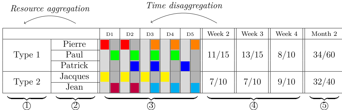
FIG. 1: Example of planning with time and resource aggregation/disaggregation. Note: every day contains 2 work shifts (light grey for AM, dark grey for PM). ① Pools: A pool is a set of resources providing a service (e.g., a specific machine) or a skillset (e.g., a team of operators), ② Operators: an operator is an elementary disjunctive resource, ③ Current week: task-period-operator links are done, ④ Weeks 2 to 4: resources are allocated for the week according to the workload, ⑤ Next month: total resource capacity is defined for the whole month. In weeks and months cells, the first number is the total amount of workload over the corresponding period. The second number is the total amount of resources allocated to the period, here the number of shifts worked by operators (Paul is off during week 4)).
