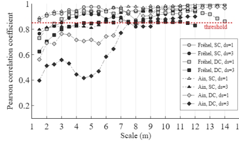
Figure 3: Linear correlation between features computed at scales separated by ds=1 m or ds=3 m for different families of features. SC = Single Cloud ; DC = Dual Cloud
