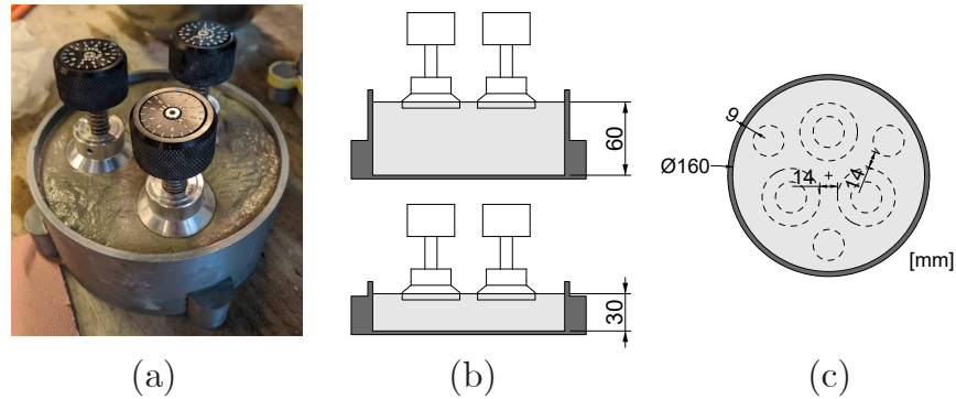
Figure 9: The ex-situ measuring device with three pocket scissometers, (b) two container heights are tested, (c) top view of the container and position of the 2 sets of 3 tests in dotted line.
