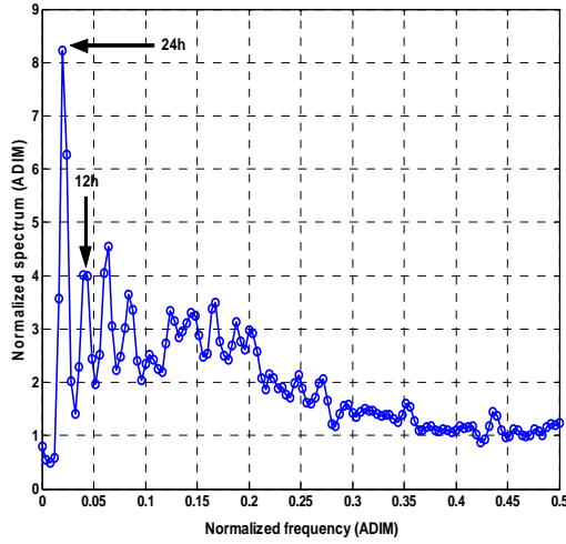
Fig. 16. Reduced spectrum of \Delta P P_1(t) ( \Delta p_{REL}(t) ), first difference of relative pore pressure P P_1(t) [kPa] at Mont Terri. Time span \sim 15 months (29/01/2004 to 12/04/2005). Time step of pre-processed signal: \Delta t = 30 min (no sub-sampling).
