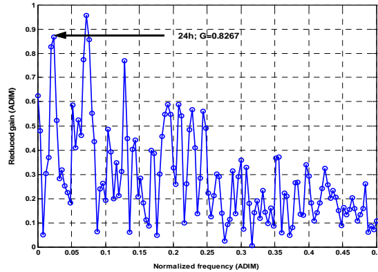
Fig. 14. Reduced spectral gain vs. normalized frequency f \times \Delta t (the maximum value of f \times \Delta t is 0.5, in agreement with Shannon's sampling theorem). This spectral gain function was obtained by cross-spectral analysis of the raw signals of atmospheric pressure P_{\text{atm}}(t) [kPa] and relative pore pressure PP1(t) - P_{\text{atm}}(t) [kPa]. Signal duration: about 1 month (from 02/08/2002 to 04/09/2002). Time step: 30 mn. The gain at diurnal frequency (1/24h) is indicated by the arrow; it is used to estimate barometric efficiency.
