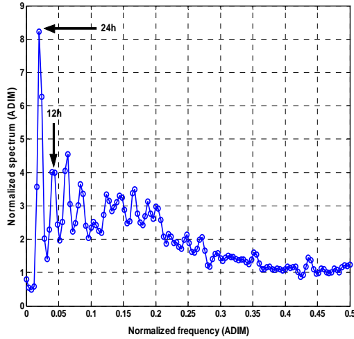
Fig. 16. Reduced spectrum of \Delta PP1(t) ( \Delta p_{REL}(t) ), first difference of relative pore pressure PP1(t) [kPa] at Mont Terri. Time span ~15 months (29/01/2004 to 12/04/2005). Time step of pre-processed signal: \Delta t=30 min (no sub-sampling).
