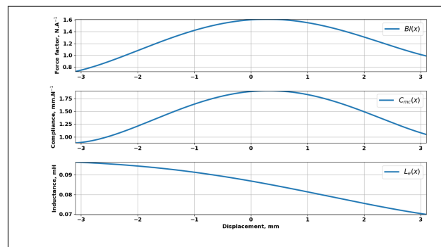
Figure 2. Dependence of the Bl factor (upper graph), compliance C_{mc} , (middle graph) and inductance L_e (lower graph) for one the loudspeaker units used in this work.
