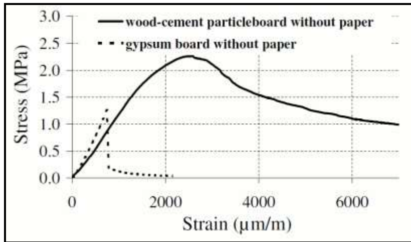
Figure 1: Characteristic stress-strain curve for a three-point bending test of wood-cement particleboard and gypsum board without paper.
