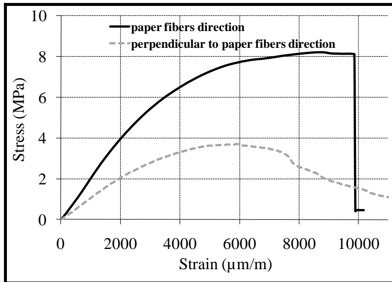
Figure 2: Characteristic stress-strain curve for a three-point bending test of wood-cement particleboard with finishing paper.
