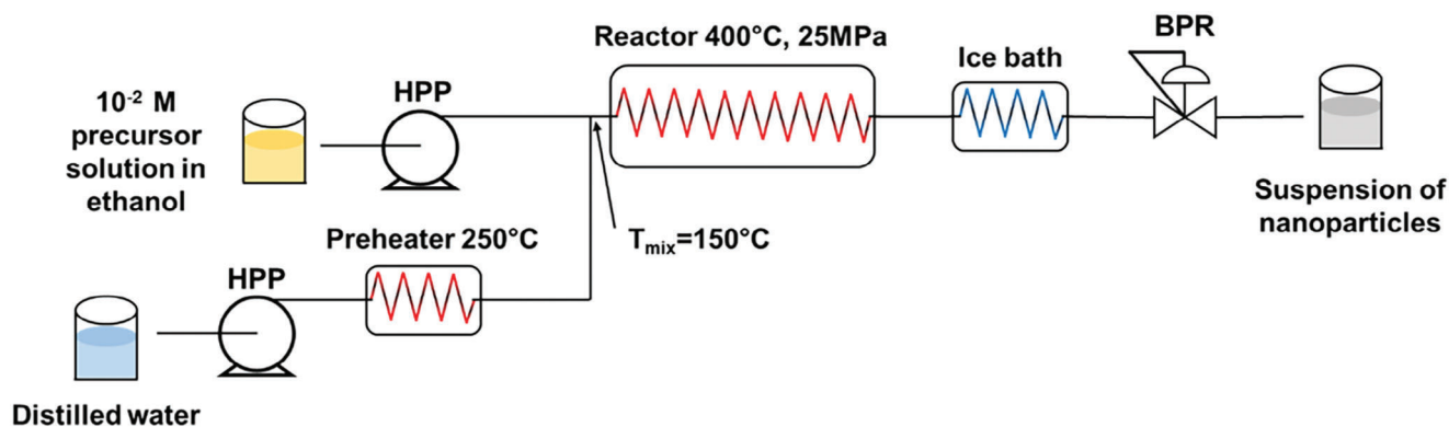
Figure 12. Continuous flow set-up used in this study for the synthesis of x\text{Y}_2\text{O}_3\text{--ZrO}_2 nanoparticles ( x = 1.5, 3 , and 8 \text{ mol.}\% \text{ Y}_2\text{O}_3 ). HPP stands for high pressure pump and BPR for back pressure regulator.
