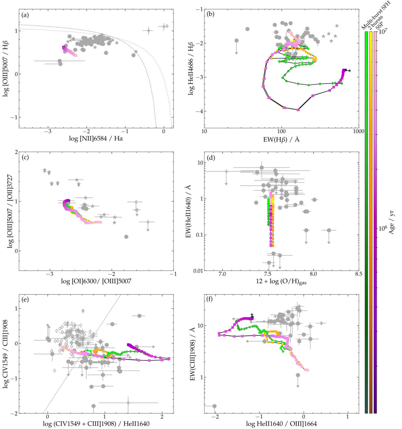
Figure 8. Same as Fig. 3, for three GALSEVN binary-star models with metallicity Z = 0.001 and the standard nebular parameters of Table 1: a plain SSP model (in green, with filled squares); one with a second burst of star formation of same amplitude as the first one added at the age of 3 Myr (in orange, with filled triangles); and one with the star formation history of a typical galaxy experiencing several bursts of different amplitudes at ages up to 10 Myr in the SPHINX cosmological simulations of Rosdahl et al. (2022, in green, with filled crosses; see the text for details).
