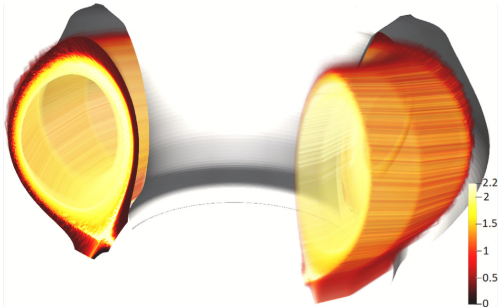
Figure 8: Grillix simulation for a 3D attached L-mode discharge in ASDEX-Upgrade at scale 1. Density fluctuations in [10^{19}m^3] . Grid of about 7 millions points, dt = 5 \times 10^{-5}R_0/C_s = 1.2ns chosen slightly below the stability limit. The model includes a third order hyperviscosity. Extracted from [116].
