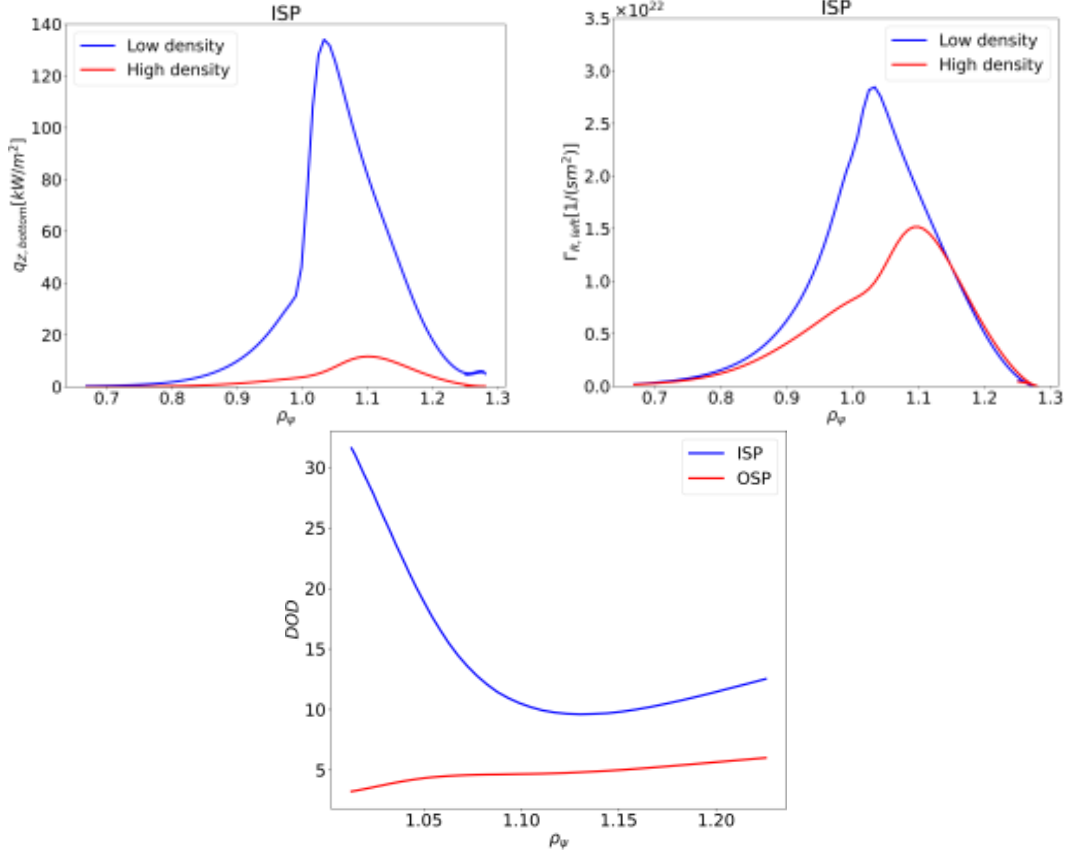
Figure 11: GBS simulations of TCV with impurities showing a detached regime at the divertor inner target. Top Left: Time- and toroidally-averaged heat flux. Top right: Time- and toroidally-averaged ion particle flux. Bottom: Degree of Detachment DOD, for flux tube at different locations, in the high-density simulation. DOD > 1 corresponds to a detached plasma [118]. Extracted and modified from [72].
