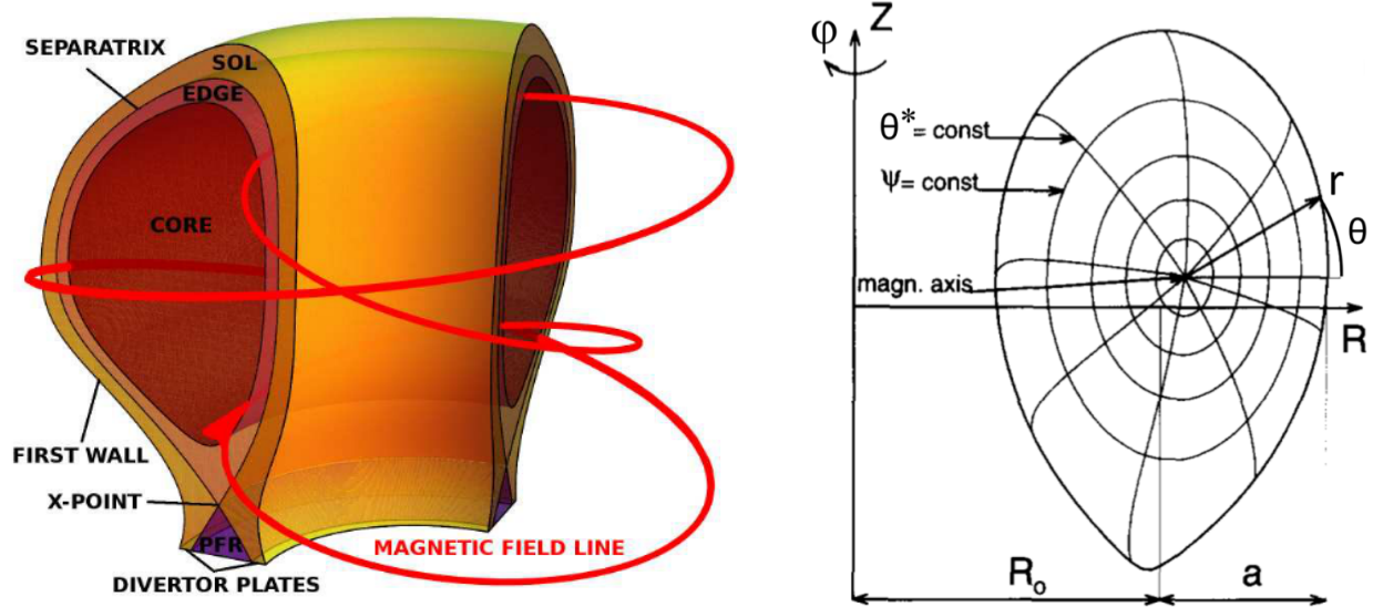
Figure 1: Sketch of the diverted plasma geometry in a tokamak. (left) Toroidal topology of a tokamak plasma, which can be categorised into the core, the edge, the scrape-off layer (SOL) and the private flux region (PFR). The separatrix separates the closed flux-surface edge region from the SOL and PFR regions, where plasma streaming along open magnetic field lines is bounded by the divertor plates. The outer SOL is also limited by the first wall. In the core and edge the magnetic field lines are either closed, fill a poloidal flux-surface or volume of space (extracted from [37]). (right) Coordinates system and geometrical parameters R_0 be the major radius, a the minor radius on the magnetic axis and (R, Z, \varphi) a fixed cylindrical coordinates system. (\psi, \theta^*, \varphi) curvilinear system of coordinates (extracted and modified from [38]).
